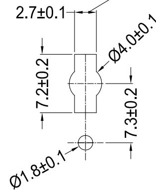
Mounting Hole Detail
