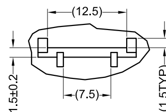
RECOMMENDED RIB DIMENSIONS (FOR REFERENCE ONLY)
